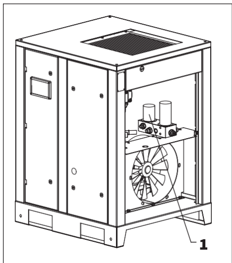
Fig. 5.4.1 Oil replacing
