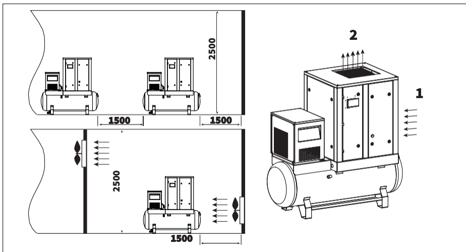
Fig. 3.3.2 Installation facility proposal AR07...AR22, ARD
